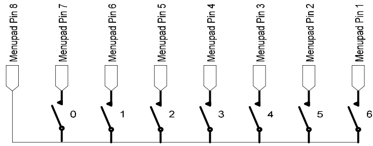
Debounce Wiring
